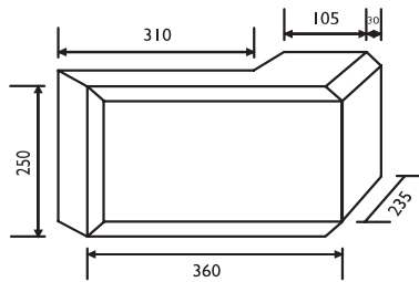
3 Brick 135 ° Full Quoin Q115A (Made to order )
